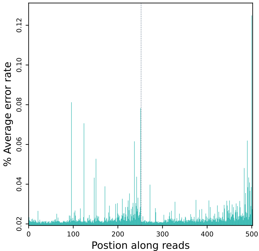
Error rate distribution along reads (R10509)
